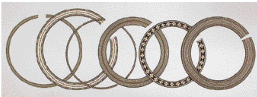
P Q R S T U
